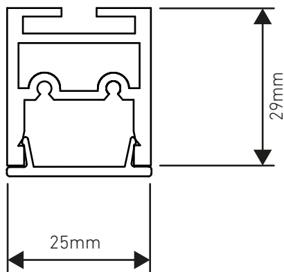
Direct Flush Diffuser
