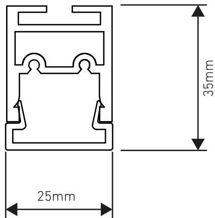
Direct Drop Diffuser
