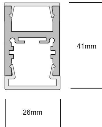
FLAT/DROP LENS
