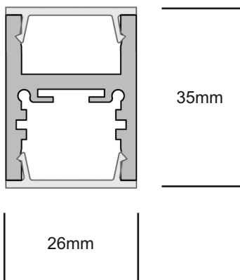
FLAT/FLAT LENS
