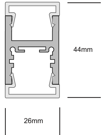
DROP/DROP LENS
