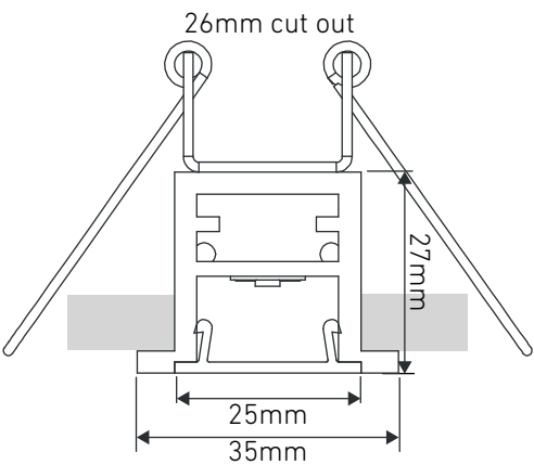
Direct Flat Trim
