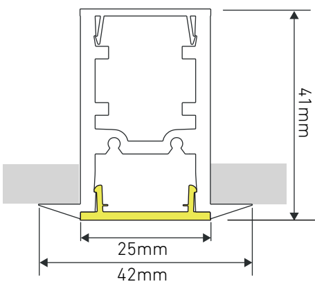
Direct Tapered Trim
