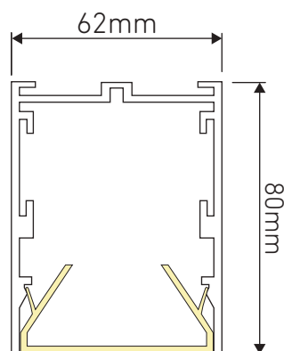
Direct Flush Diffuser
