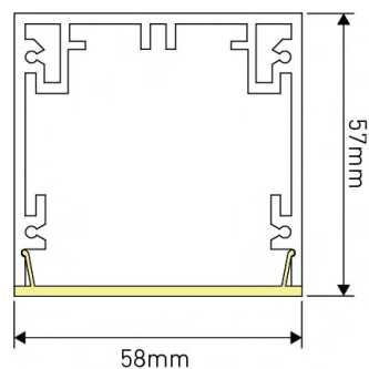
Direct Flush Diffuser
